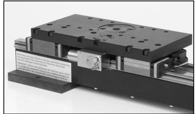
Note: For single rail 40 & 50 series bores, top and bottom plates are same as G2
